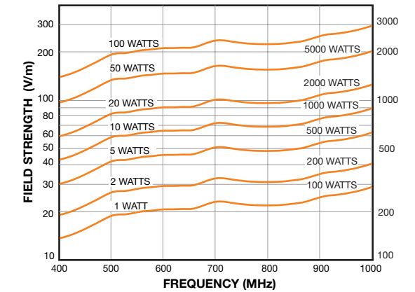
FIELD STRENGTH MEASURED AT 1 METER
