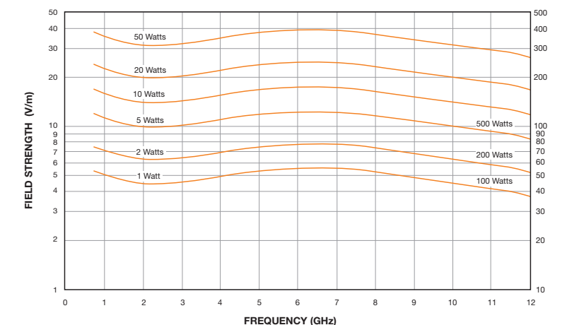
FIELD STRENGTH MEASURED AT 3 METERS
