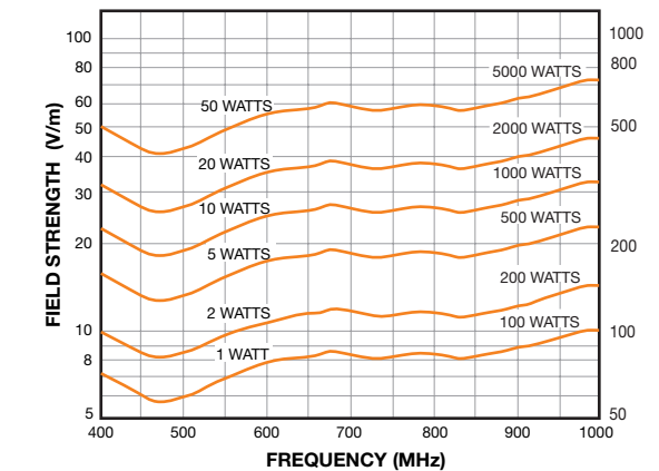
FIELD STRENGTH MEASURED AT 3 METERS
