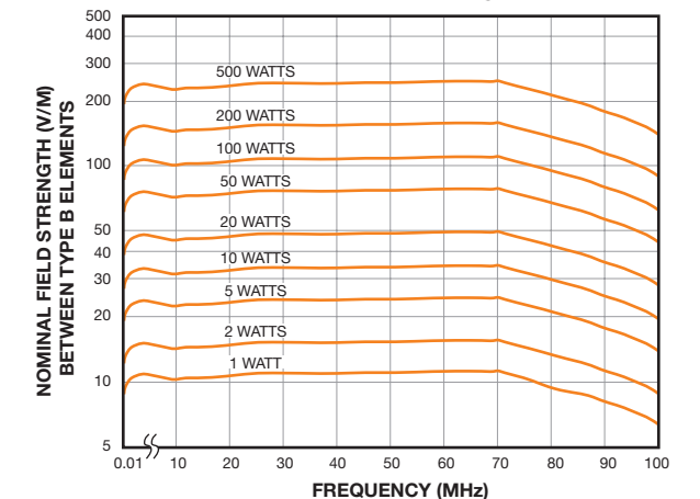
FIELD STRENGTH MEASURED BETWEEN TYPE B ELEMENTS
