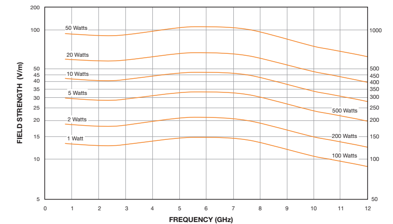
FIELD STRENGTH MEASURED AT 1 METER
