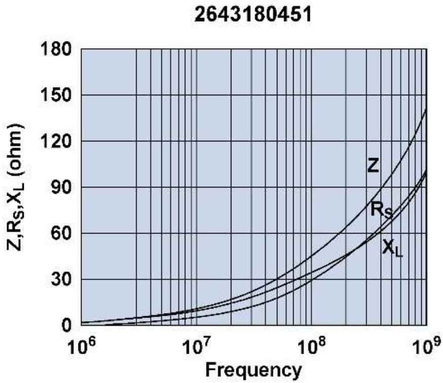
Impedance, reactance, and resistance vs. frequency.
