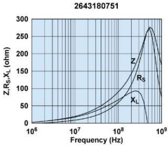
Impedance, reactance, and resistance vs. frequency.
