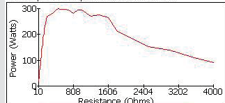
Autosequence Step 777 Power Curve Test
