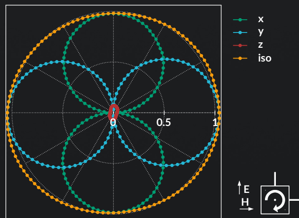
Isotropy @ 1 GHz, normalized E-field rotating in E-H-plane
