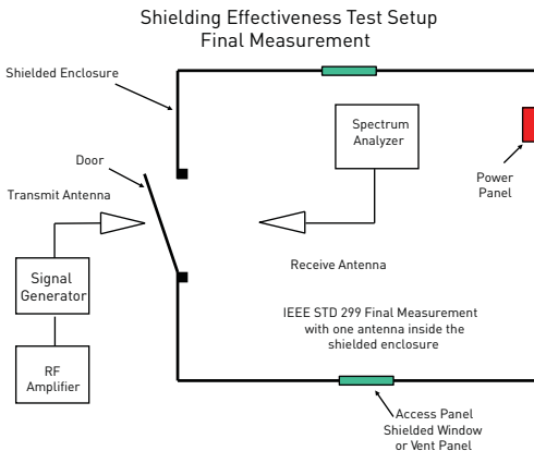
Figure 4-3. IEEE STD 299
