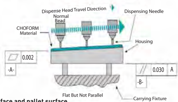
Figure 8-5 Non-parallelism between receiving surface and pallet surface
