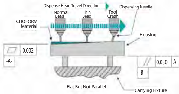
Figure 8-5 Non-parallelism between receiving surface and pallet surface
