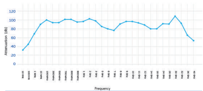
Shielding Effectiveness of Double Layer Nova™
